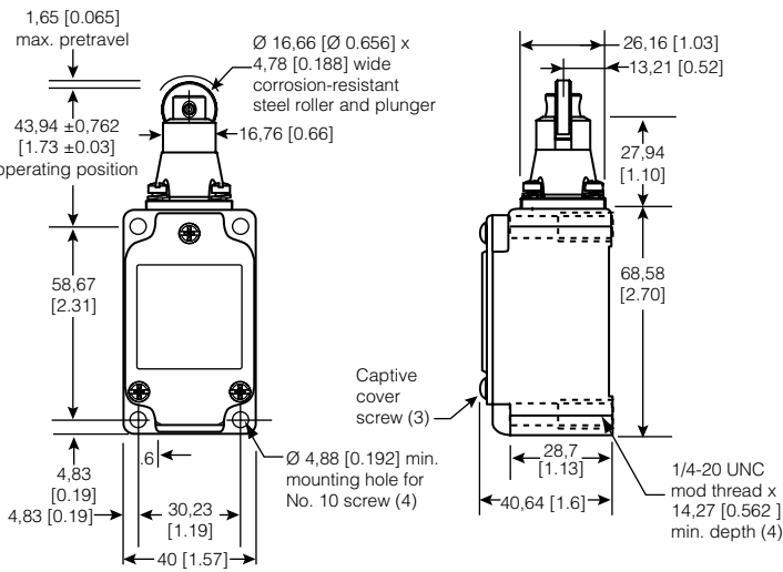
Figure 7. 5LS1 Dimensions
